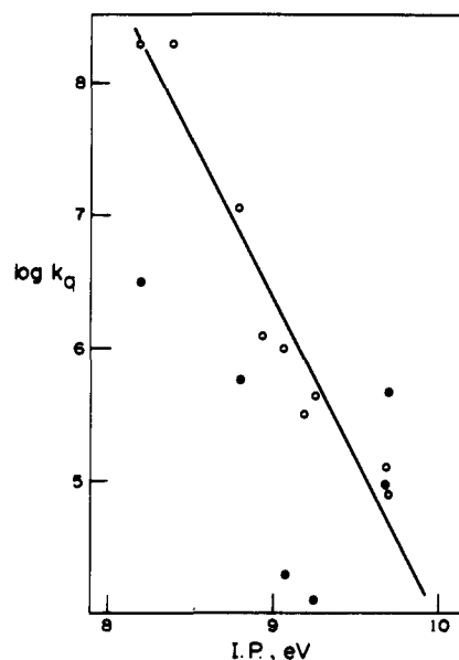
Figure 5. Dependence of quenching rate constants for substituted benzenes on their ionization potentials: \circ , triplet AF 3 in CH 3 CN; \bullet , triplet benzophenone in CFC 12 CF 2 Cl, ref 6c.
