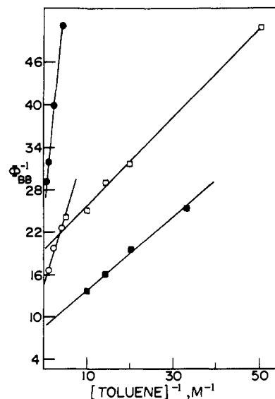
Figure 3. Double reciprocal dependence of quantum yields for bibenzyl formation on toluene concentration: \circ , AF 3 itself; \bullet , m -ClAF 3 ; \square , m -CF 3 AF 3 ; \blacksquare , p -CF 3 AF 3 .
