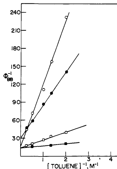
Figure 2. Double reciprocal dependence of quantum yields for bibenzyl formation on toluene concentration: \circ , p -MeOAF 3 ; \bullet , m -MeAF 3 ; \square , p -MeAF 3 ; \blacksquare , p -ClAF 3 .
