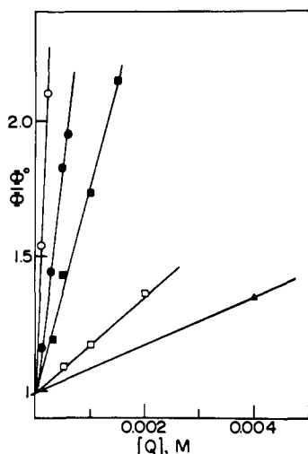
Figure 4. Representative Stern-Volmer quenching plots, naphthalene quencher, bibenzyl monitored at 1.0 M toluene, 0.05 M ketone: \circ , p -MeAF 3 ; \bullet , p -ClAF 3 ; \blacksquare , AF 3 itself; \square , m -ClAF 3 ; \triangle , p -CF 3 AF 3 (0.1 M toluene, other points off graph).
